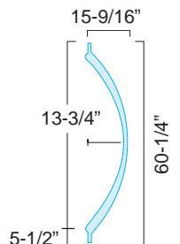
DW1922 $402.00 ea. 60" Dia x 14" Deep x 5-1/2" Rim
